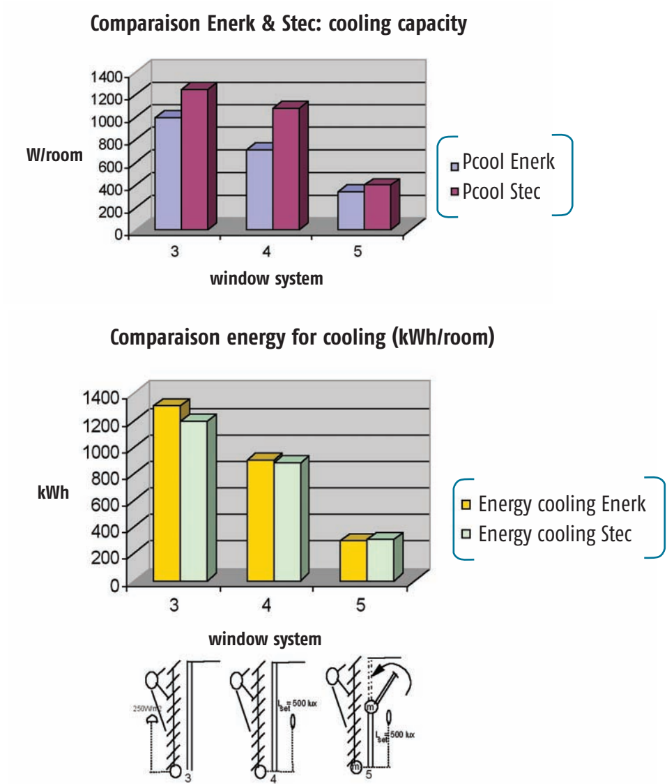
Figure A1 . Cooling load capacity and energy consumption for cooling calculated by two different programs: Enerk and Stec [PhD, Stec]
