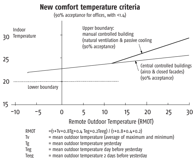
Figure 1.1 Adaptive comfort criterion as proposed in The Netherlands.
