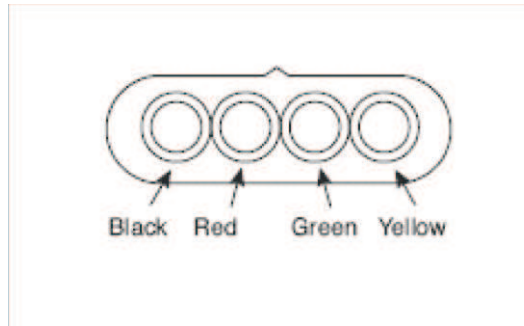
4 Conductor Modular Cable with RJ9 Connectors
